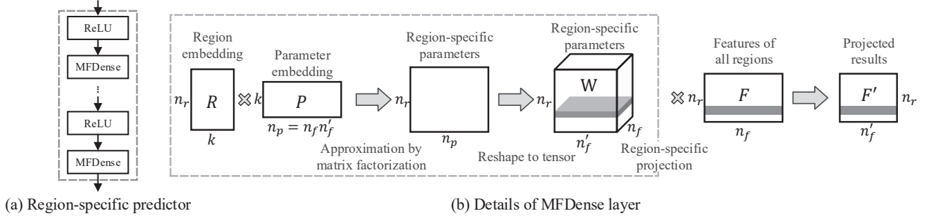
Figure 4: Detail structure of region-specific predictor.
