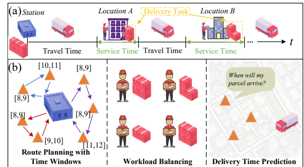
Figure 1: Service Time and Its Applications.
