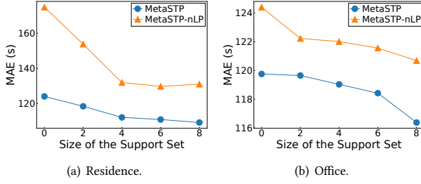
Figure 7: Different # of Support Observations.
