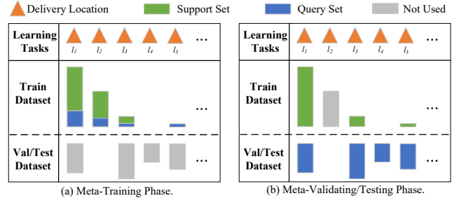
Figure 4: Illustration of Learning Task Setup.
