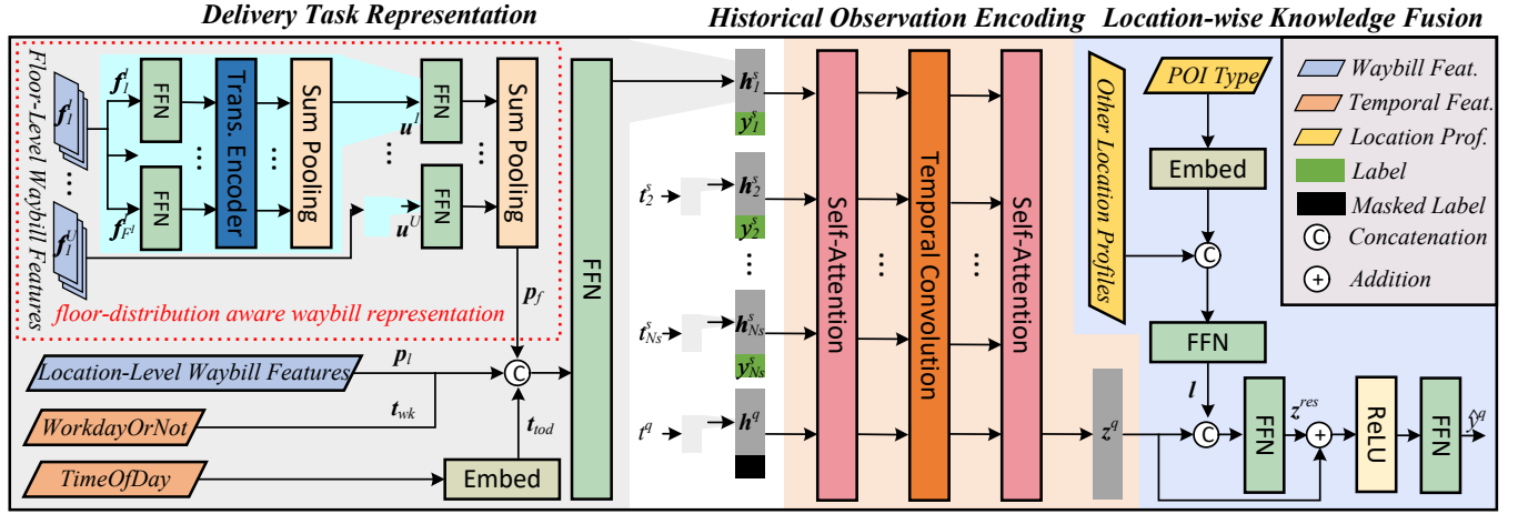
Figure 5: The Architecture of MetaSTP.
