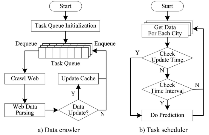
Fig. 5. Procedure of data crawler and task scheduler.
