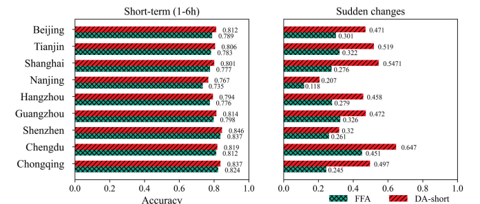
Fig. 12. Comparison with previous online model on nine Chinese cities.
