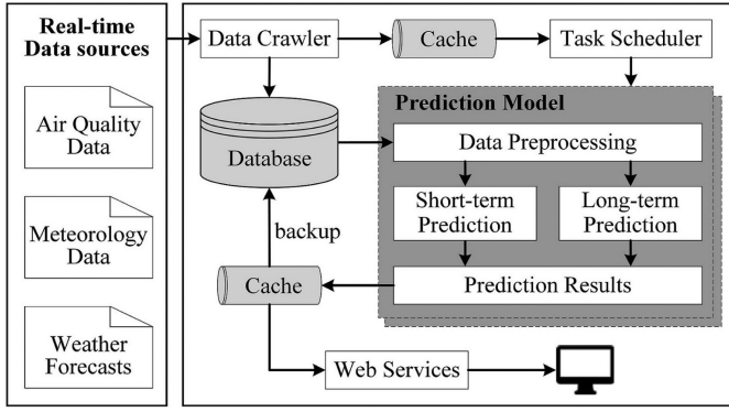
Fig. 4. Architecture of air quality prediction system.
