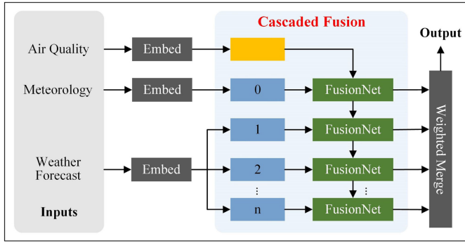
Fig. 9. Framework of city-level long-term prediction.
