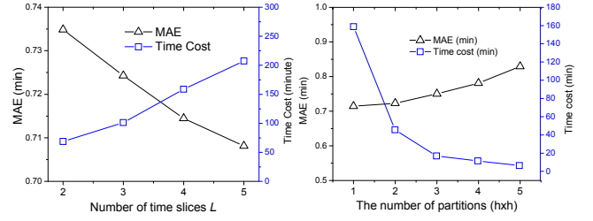
A) W.r.t. time slices B) w.r.t. partitions Figure 12. Performance of CATD
